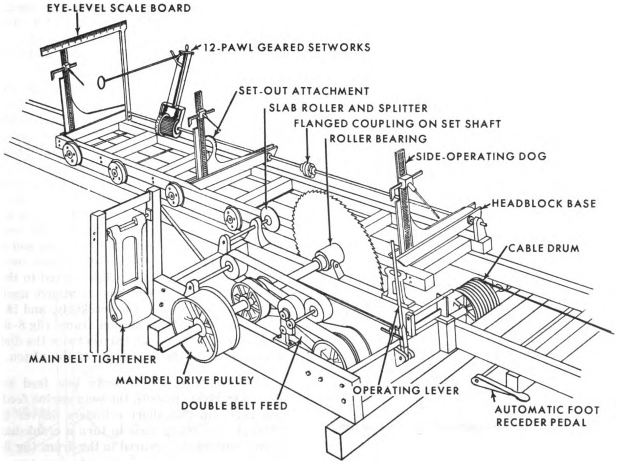
Figure 8-3. Headblock type sawmill.
